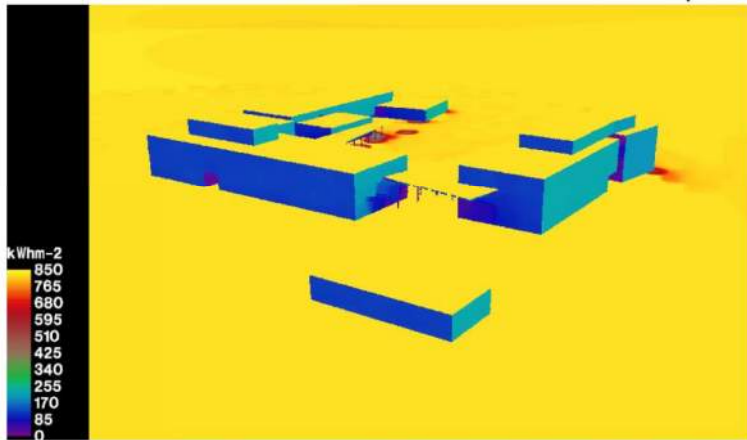
Solar Radiation from April to October (10:00 am - 05:00 pm) North Perspective
