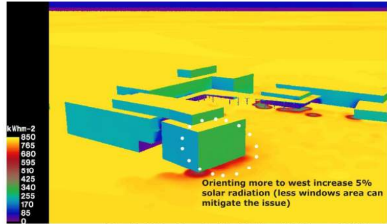
Solar Radiation from April to October (10:00 am - 05:00 pm) West Perspective
