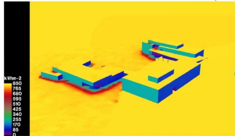
Solar Radiation from April to October (10:00 am - 05:00 pm) East Perspective
